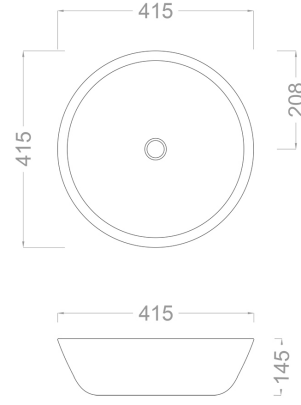
TECHNICAL DRAWING
