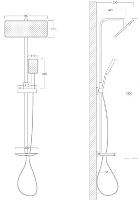
TECHNICAL DRAWING
