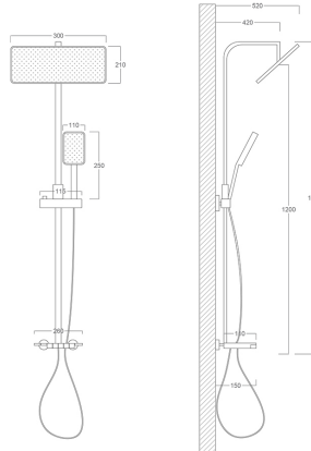
TECHNICAL DRAWING
