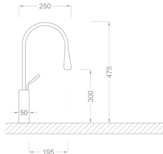
TECHNICAL DRAWING
