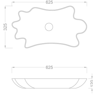
TECHNICAL DRAWING
