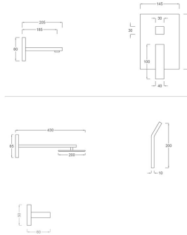
TECHNICAL DRAWING
