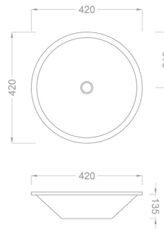
TECHNICAL DRAWING
