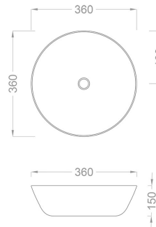
TECHNICAL DRAWING
