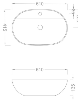
TECHNICAL DRAWING
