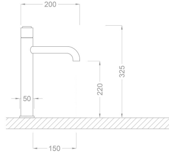
TECHNICAL DRAWING
