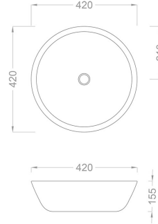
TECHNICAL DRAWING
