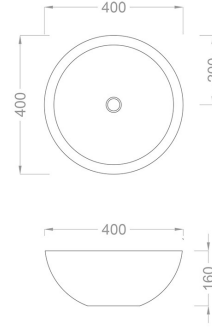
TECHNICAL DRAWING
