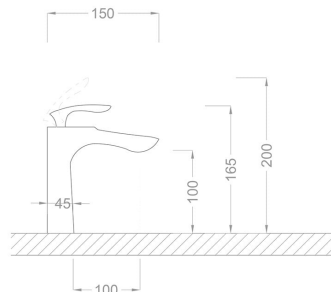
TECHNICAL DRAWING
